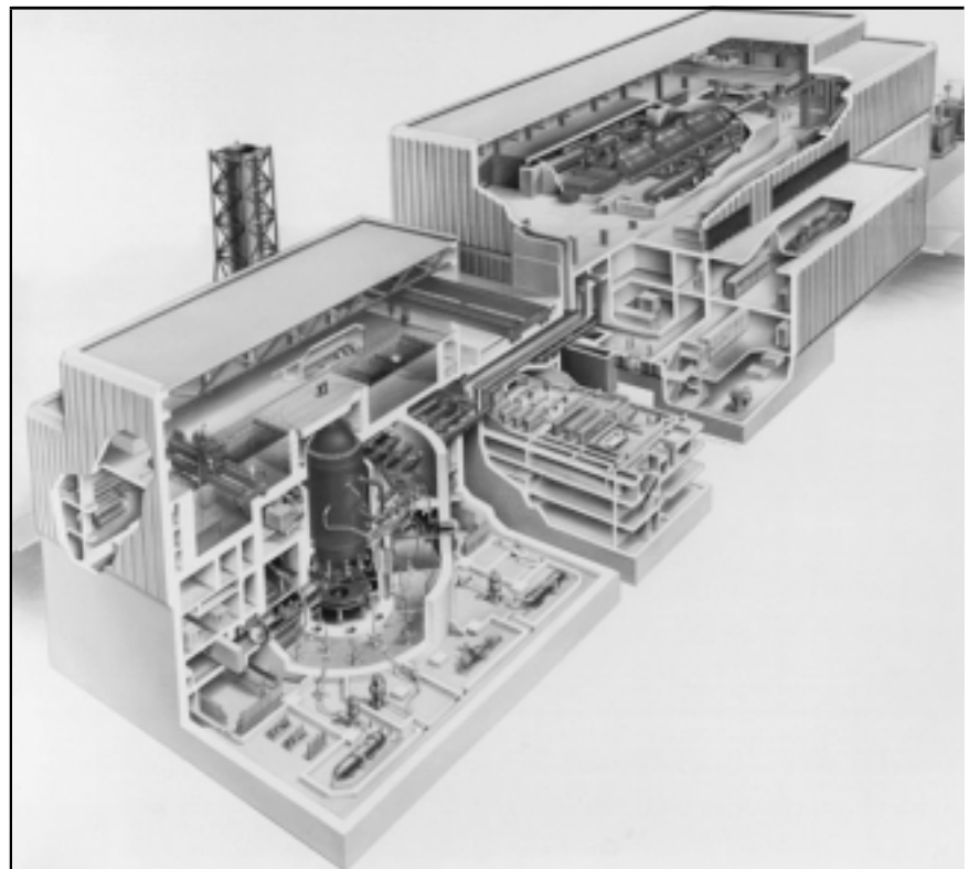
FIGURE 4 General Electric's ABWR
