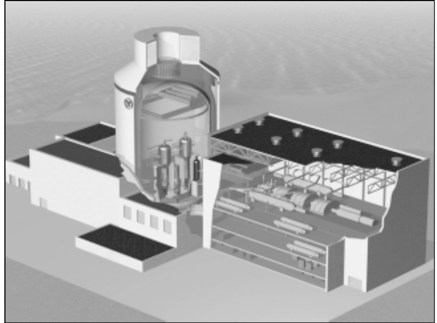
FIGURE 3 Westinghouse AP1000
