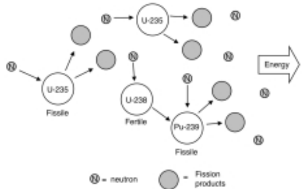
FIGURE 2 Simplified Diagram of the Uranium Fuel Cycle
