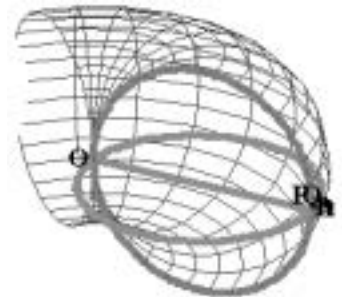
Computer graphic representation of torus.
