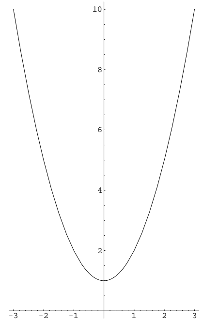
Equation X = x^2 + 1 :
