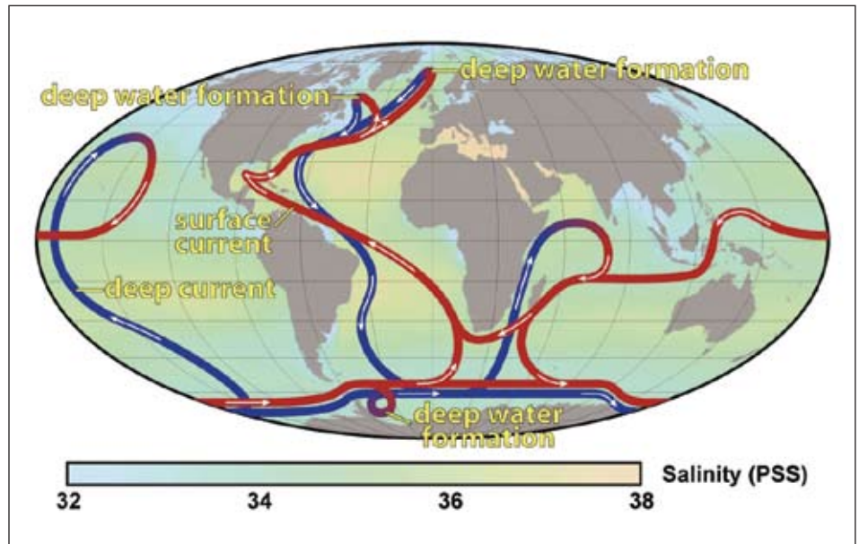
FIGURE 5 Thermohaline Circulation
