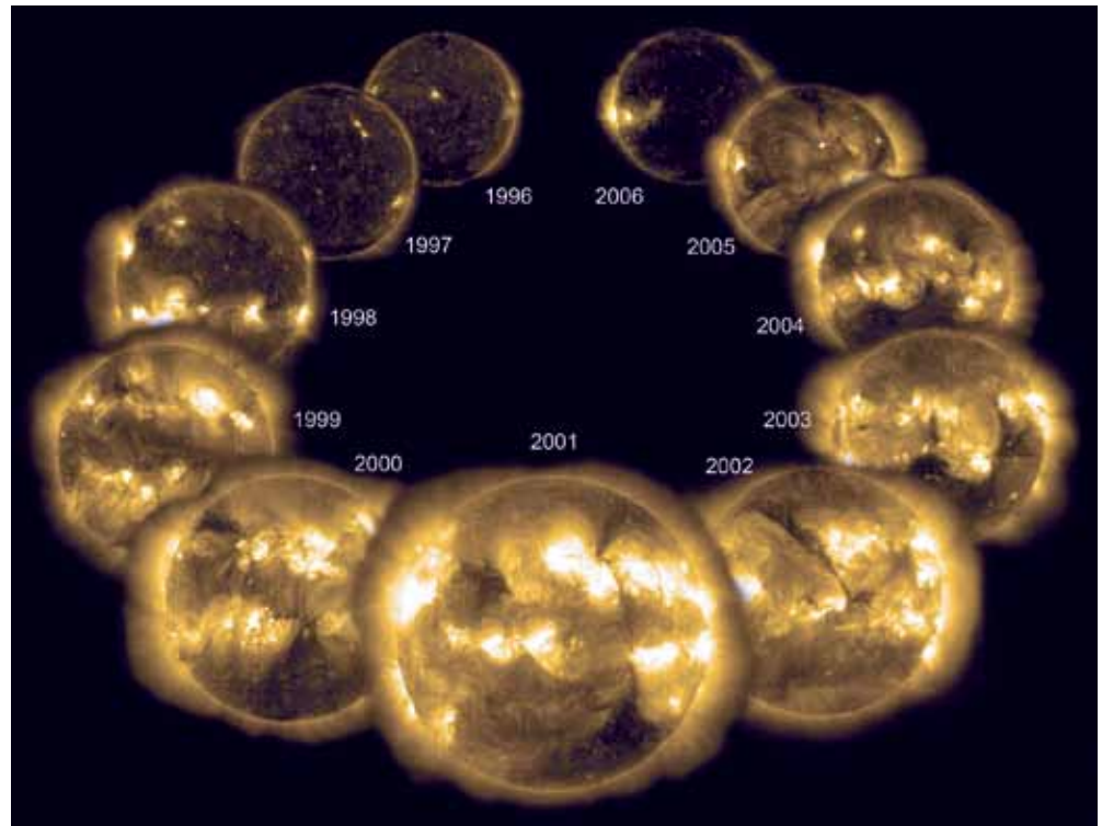
Steele Hill, SOHO, NASA/ESA Year by year X-ray images of the Sun as it progresses through an eleven year cycle (starting weak in 1996, peaking in 2001, and ending weak in 2006).
