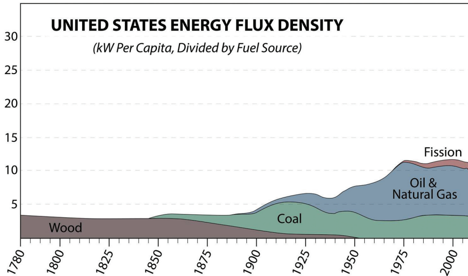
The per-mass energy content of various energy sources. Wood, coal, and petroleum are burned to release their chemical energy. Uranium is made to undergo fission in a nuclear reactor to release nuclear energy, as does deuterium in the process of nuclear fusion. Anti-matter can be converted directly to energy as expressed by Einstein's famous relationship that E = mc^2 .
