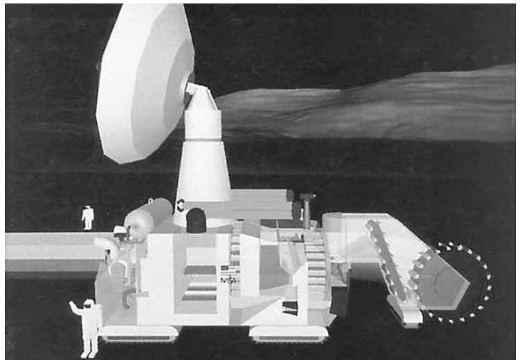
There are about 1 million tons of helium-3—a rare isotope of helium on Earth, which can be used as fusion fuel—trapped on and near the surface of the Moon. This Lunar Mark-II is a mobile robotic miner designed to process the soil, extract the helium, redeposit the processed soil, and move on. The University of Wisconsin device has a soil processing rate of 556 tons per hour.
