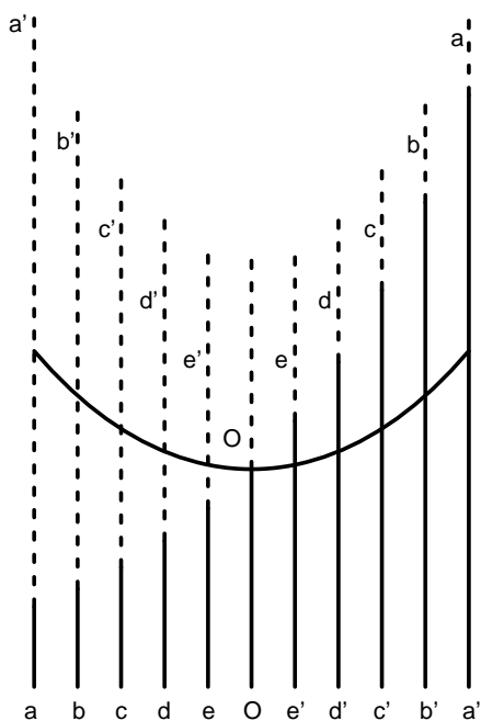
FIGURE 3 Leibniz’s Construction of the Catenary
