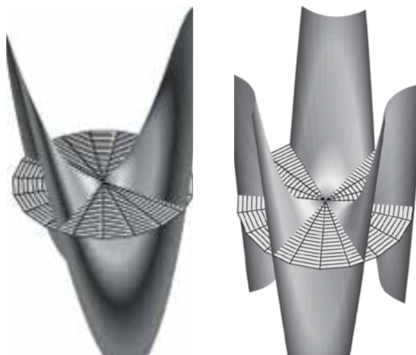
FIGURE 4 Gaussian Surfaces
