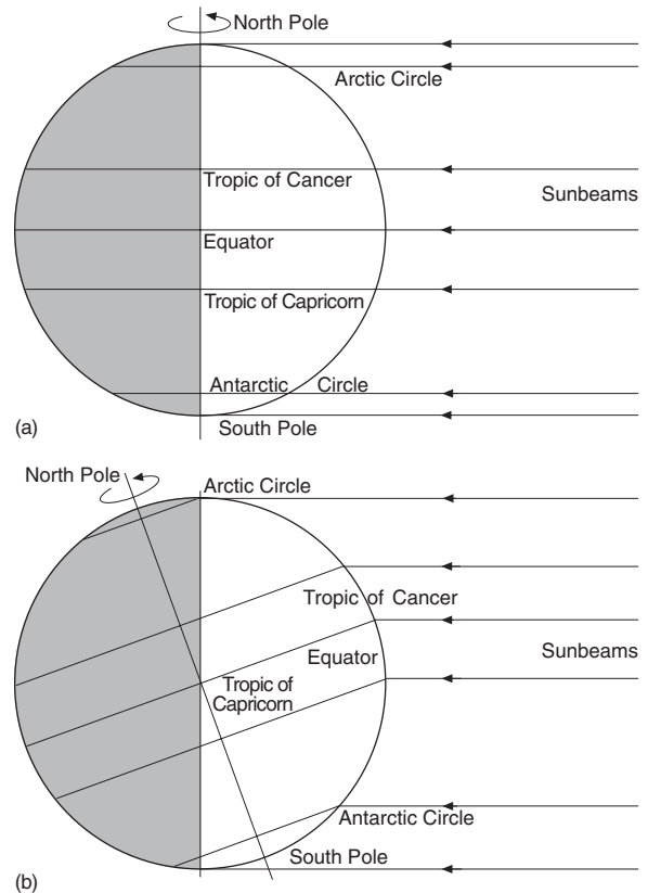
FIGURE 6 Obliquity and Intensity of the Sun's Rays
