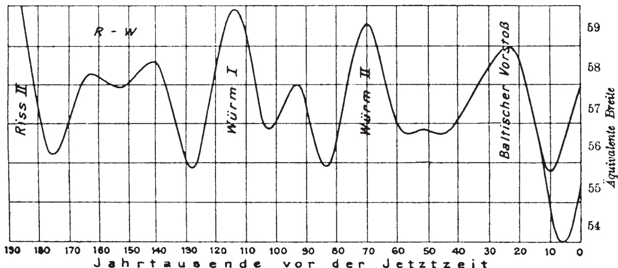
This radiation curve by Milankovitch was reproduced by Köppen and Wegener in their book Die Klimate der geologischen Vorzeit (The Climates of the Geological Past), a pioneering work in paleoclimatology published in 1924. The horizontal axis shows years (in thousands) from present; the vertical plots fluctuations in radiation.
