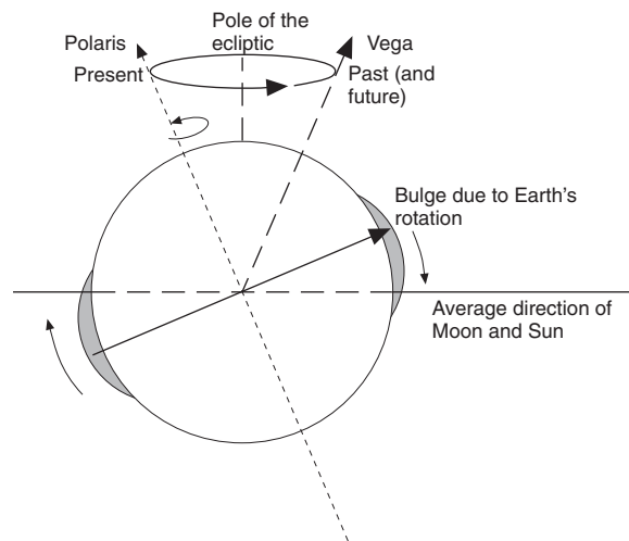
FIGURE 3 Precession and Change of Pole Star
