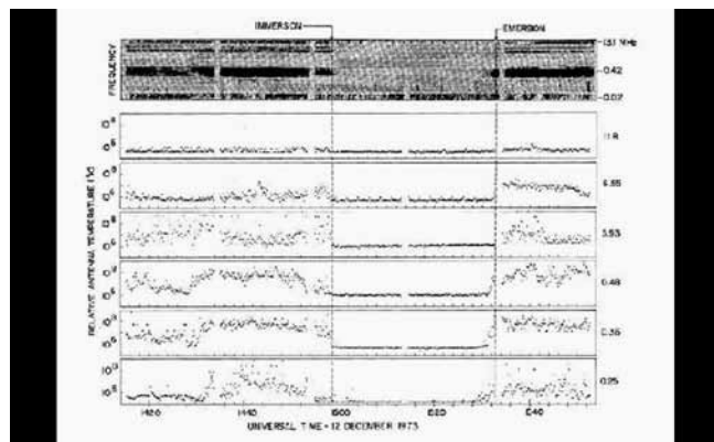
FIGURE 10 Measuring the Moon's Radio Environment
