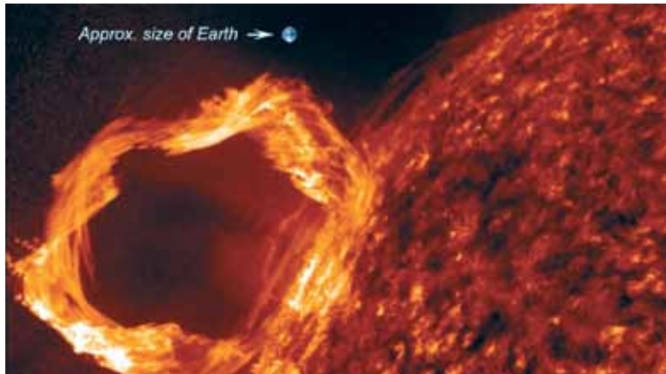
FIGURE 7 A Solar Prominence
