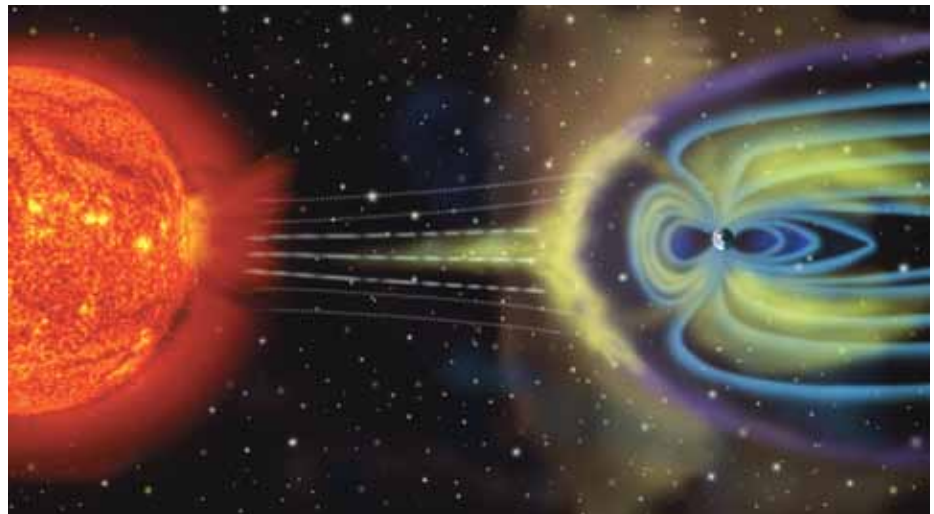
FIGURE 1 A Solar Flare Hitting the Earth's Magnetic Field
