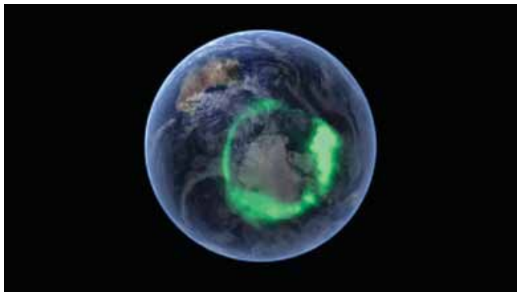
FIGURE 8 An Aurora Australis
