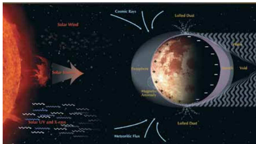
FIGURE 11 An Image of a Solar Storm Directed at the Moon
